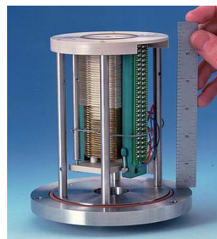
Figure 4. Electrodynamic Ion Funnel.
